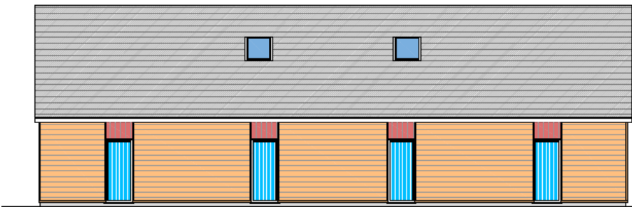
UNIT B SOUTH FACING ELEVATION
